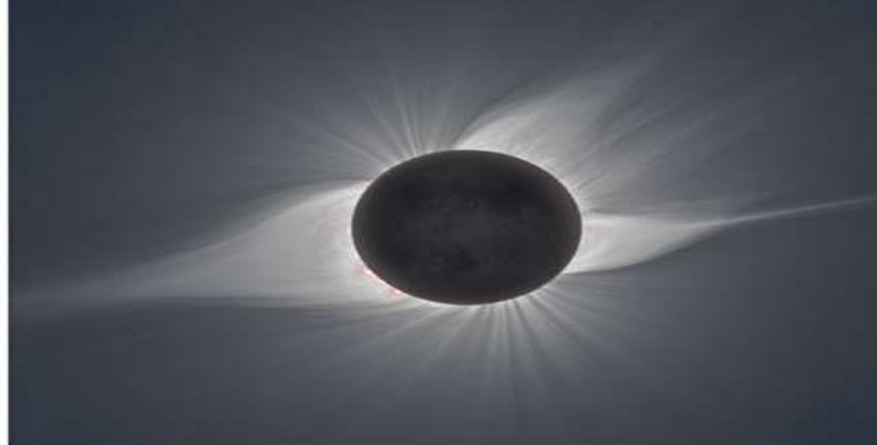
(b) corona during descending phase (1994)
