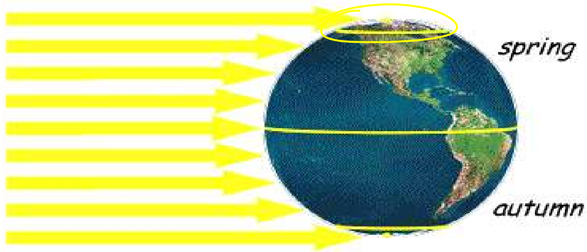
vernal equinox (March 20/21)
