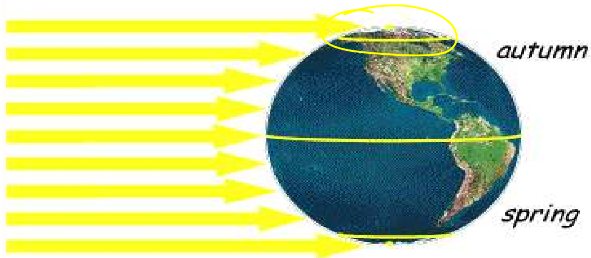
autumnal equinox (September 22/23)
