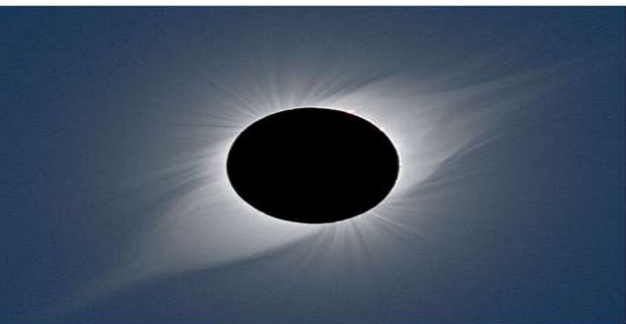
(c) solar minimum corona (1995)
