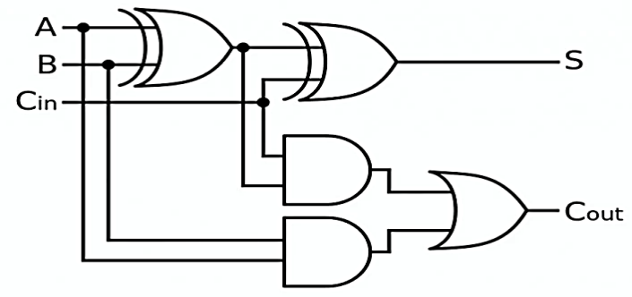
Simple Digital Circuit
